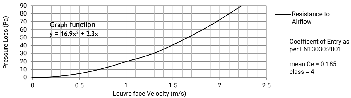
Pressure Loss Graph for 1m High Emtec Type LAAC 30-105 Acoustic Louvre
