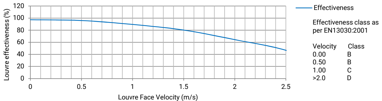
Effectiveness of Louvre with Simulated Wind and Rain for Emtec Type LAAC 30-105 Acoustic Louvre
