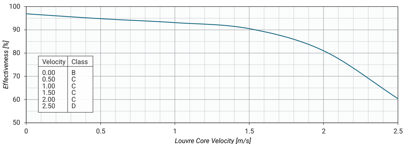
Effectiveness of Louvre with Simulated Wind and Rain for Emtec Type LSH-50-75-SE
