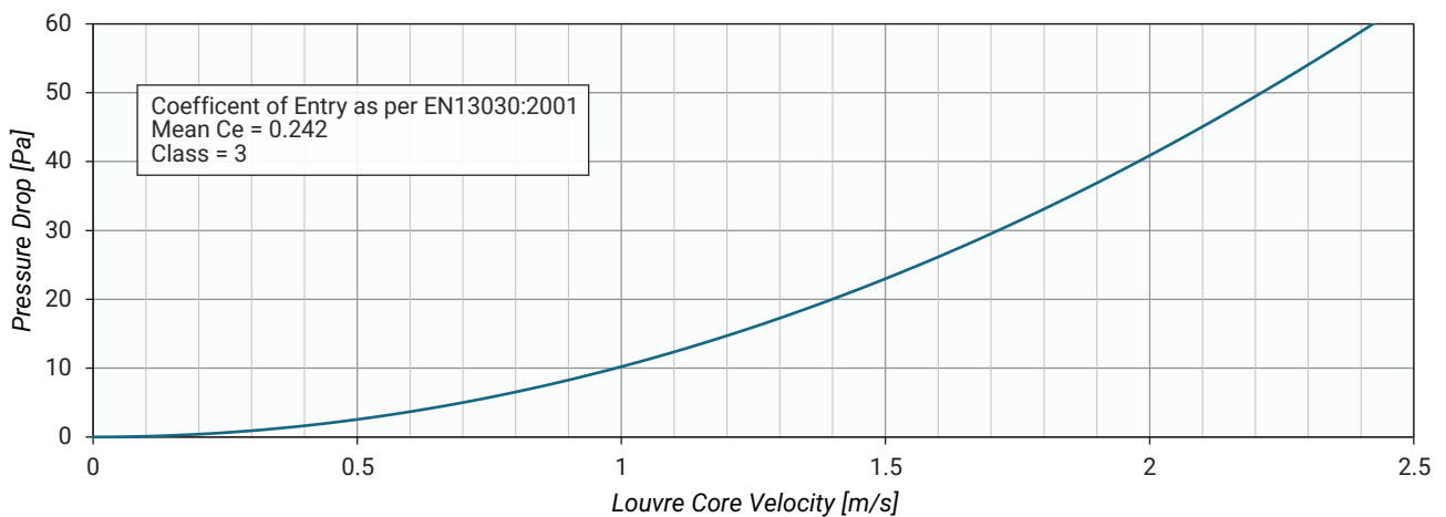
Pressure Loss Graph for 1m High Emtec Type LSH-50-75-SE
